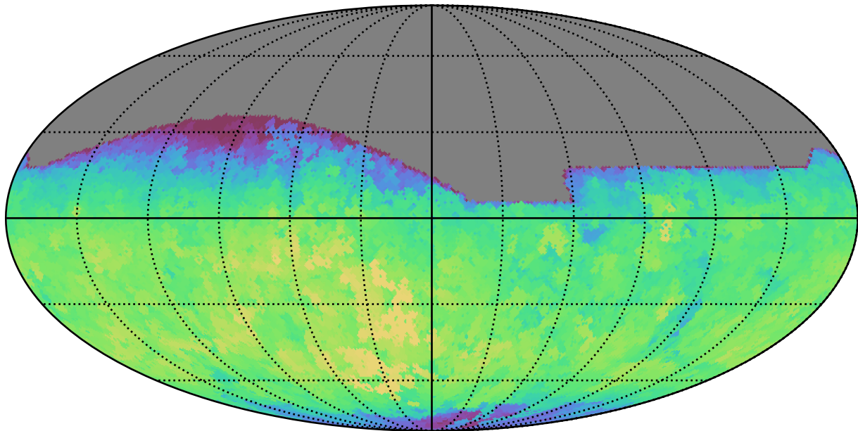
too_5_1v3.4_10yrs All sky all bands: Max fiveSigmaDepth
