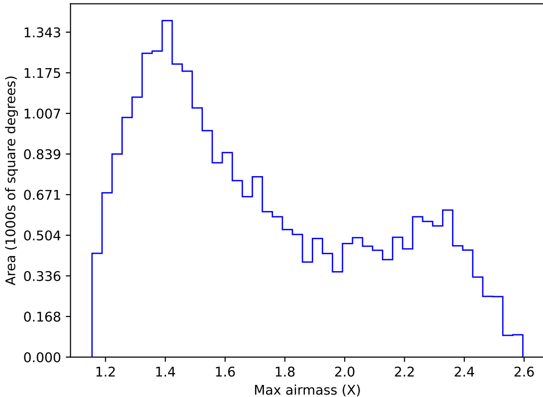
too_5_1v3.4_10yrs Yr 1 r band: Max airmass
