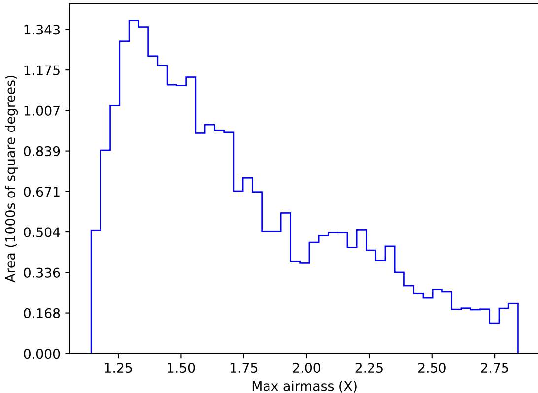
too_5_1v3.4_10yrs Yr 1 i band: Max airmass
