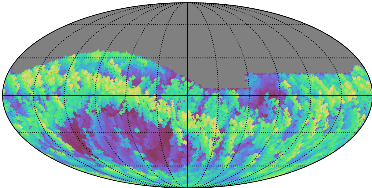
too_5_1v3.4_10yrs Yr 1 all bands: Max airmass
