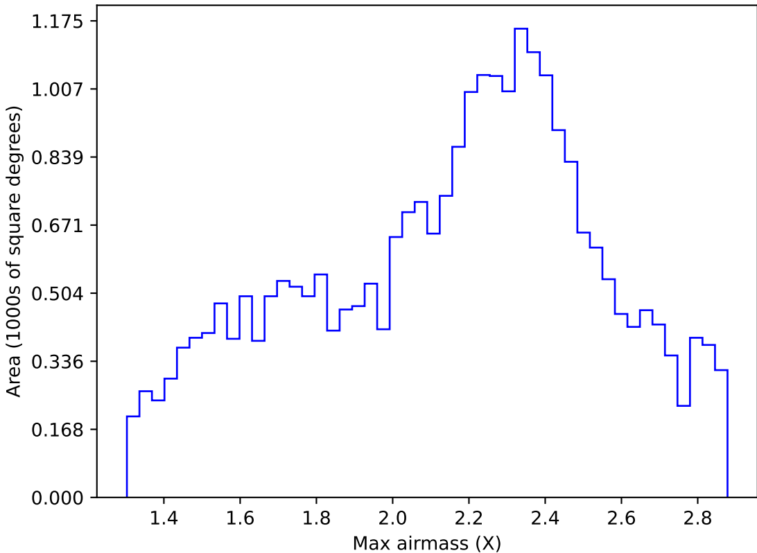
too_5_1v3.4_10yrs Yr 1 all bands: Max airmass
