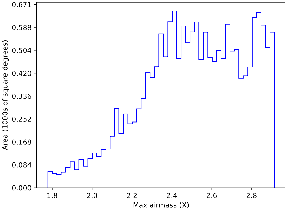
too_5_1v3.4_10yrs WFD z band: Max airmass
