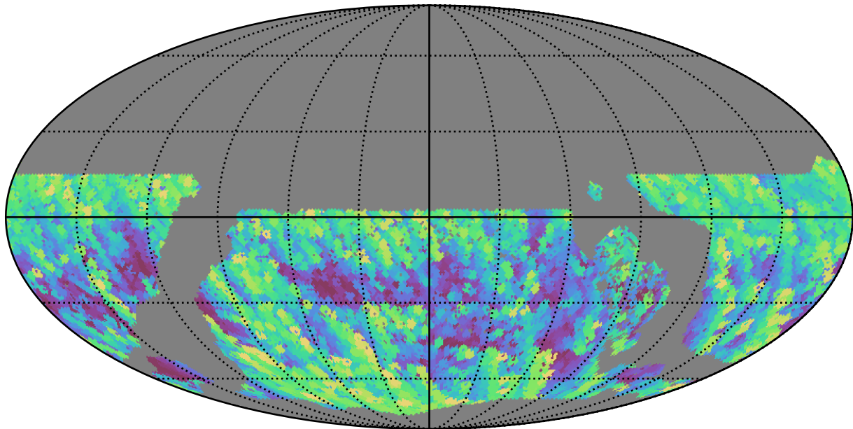
too_5_1v3.4_10yrs WFD y band: Max airmass
