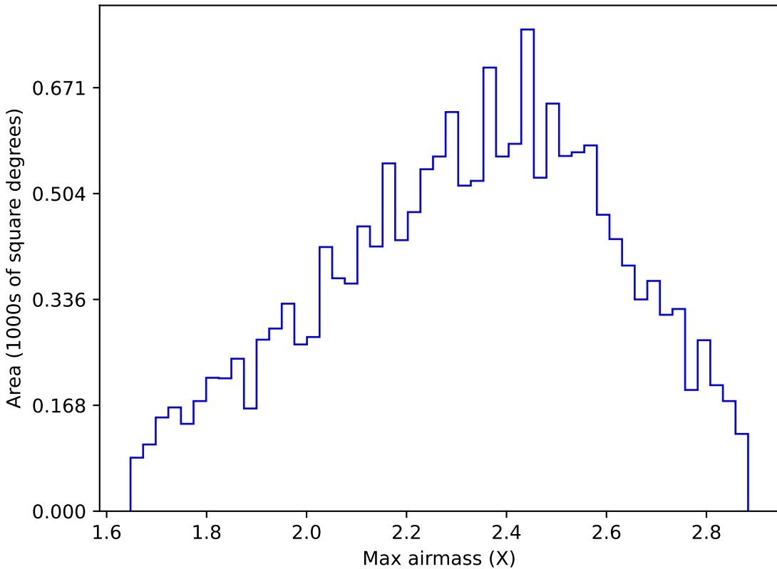
too_5_1v3.4_10yrs WFD y band: Max airmass
