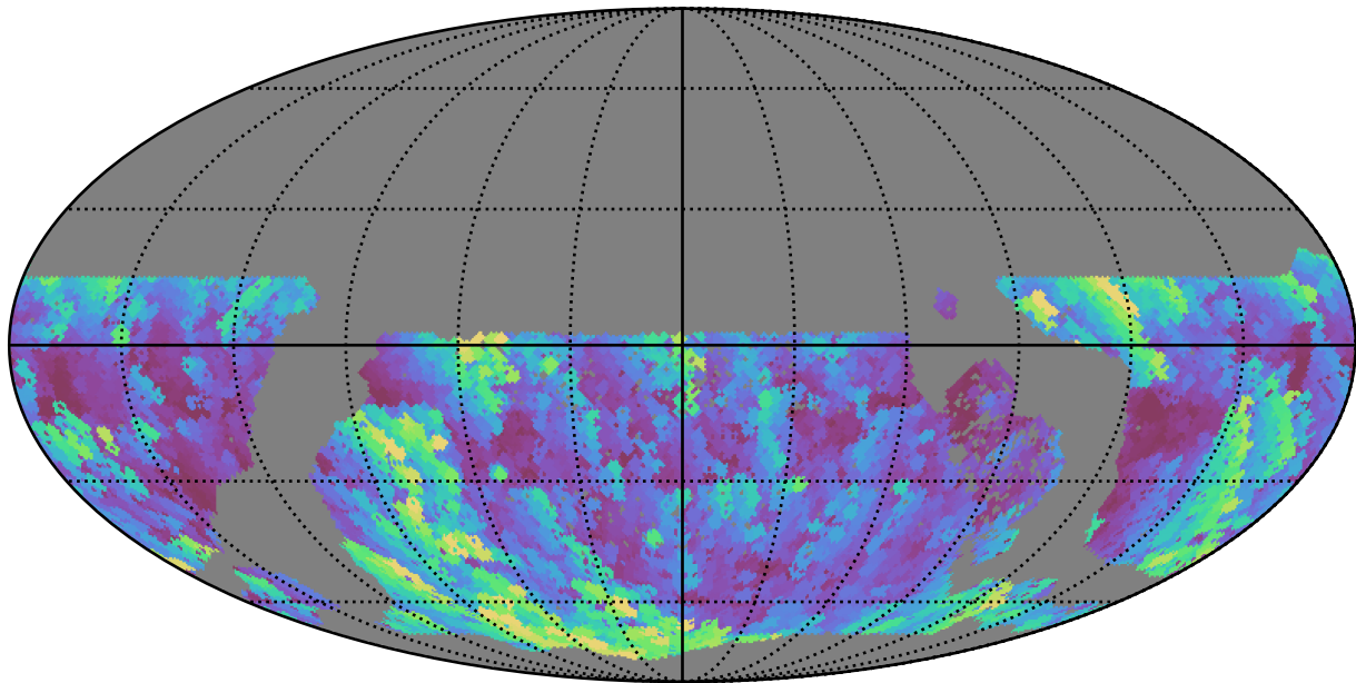
too_5_1v3.4_10yrs WFD u band: Max airmass
