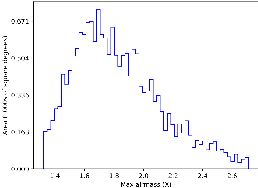
too_5_1v3.4_10yrs WFD u band: Max airmass
