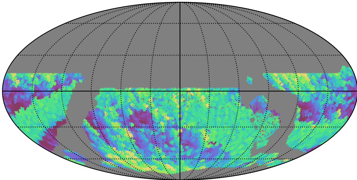
too_5_1v3.4_10yrs WFD r band: Max airmass
