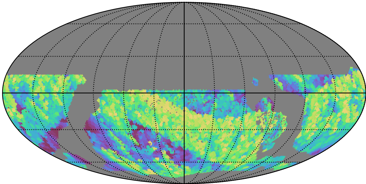
too_5_1v3.4_10yrs WFD i band: Max airmass
