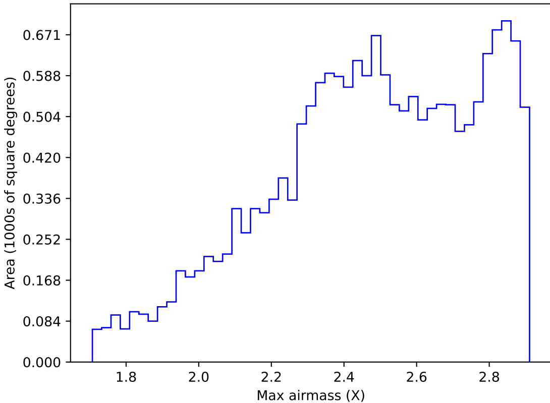
too_5_1v3.4_10yrs WFD i band: Max airmass
