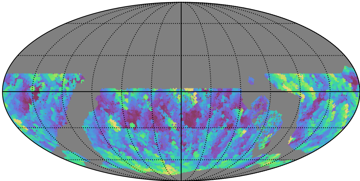
too_5_1v3.4_10yrs WFD g band: Max airmass
