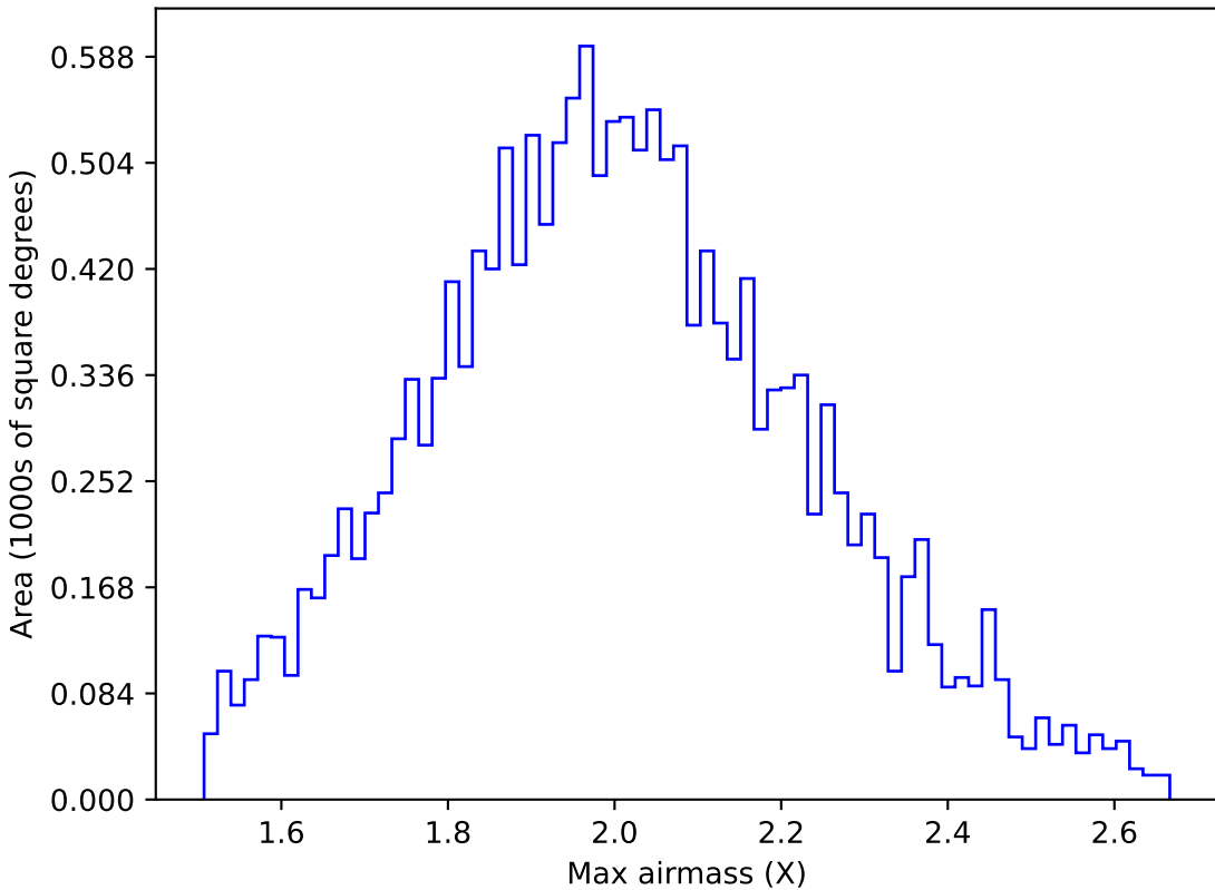
too_5_1v3.4_10yrs WFD g band: Max airmass
