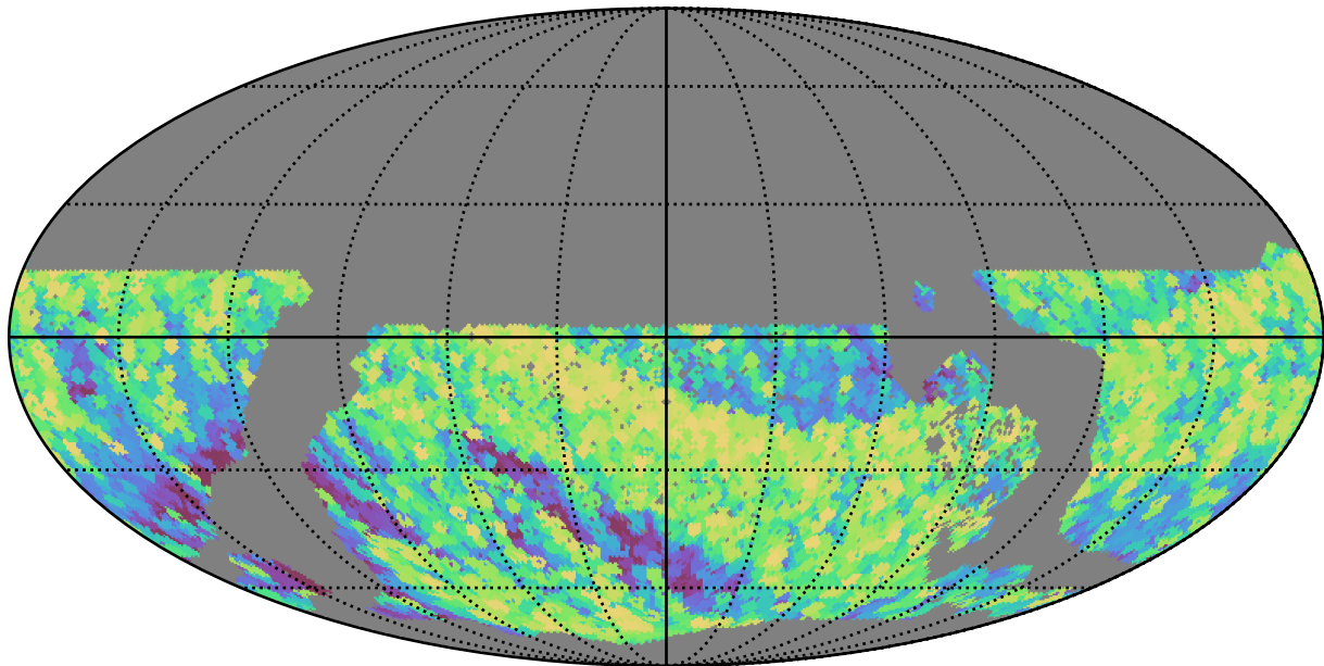
too_5_1v3.4_10yrs WFD all bands: Max airmass
