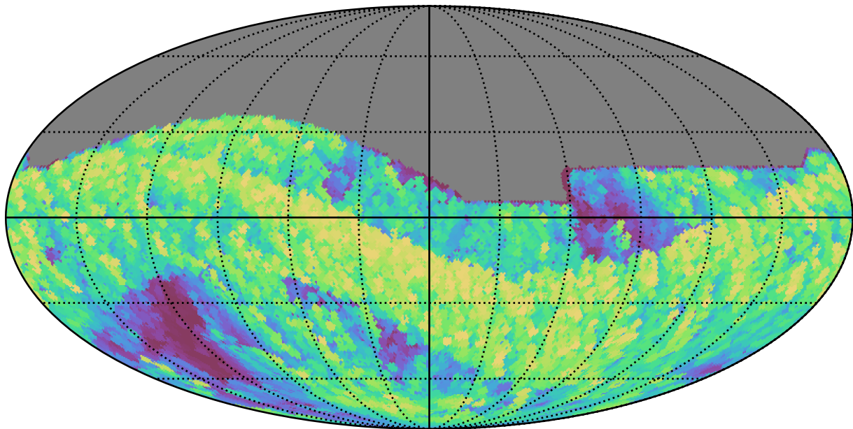
too_5_1v3.4_10yrs All sky z band: Max airmass
