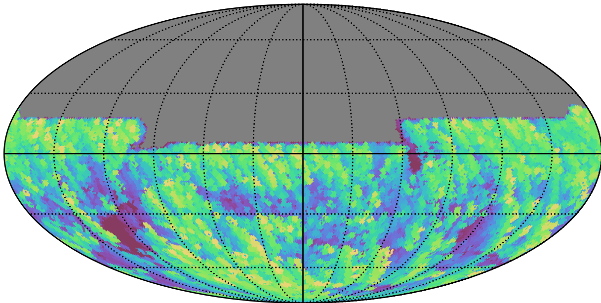
too_5_1v3.4_10yrs All sky y band: Max airmass
