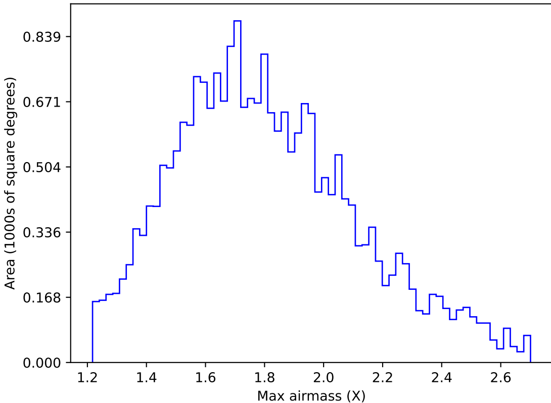
too_5_1v3.4_10yrs All sky u band: Max airmass
