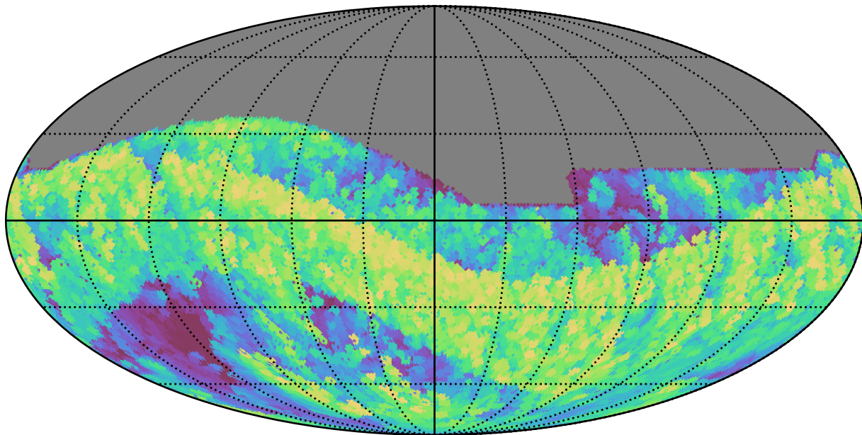
too_5_1v3.4_10yrs All sky i band: Max airmass
