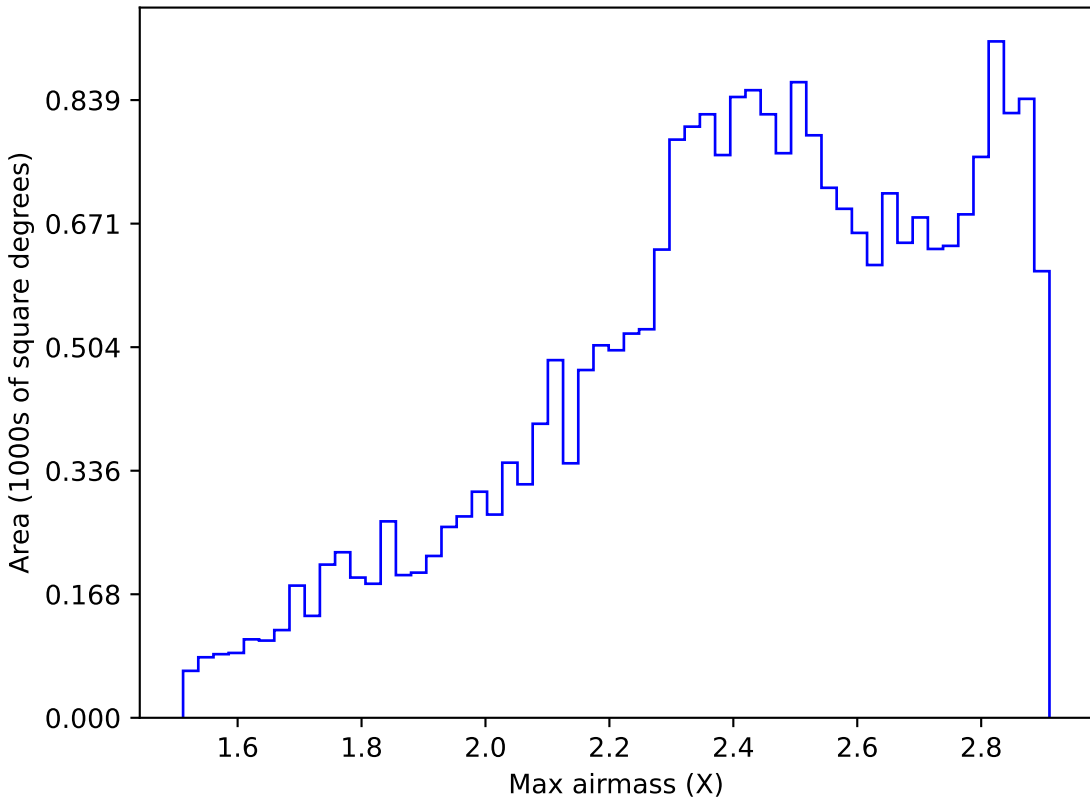
too_5_1v3.4_10yrs All sky i band: Max airmass
