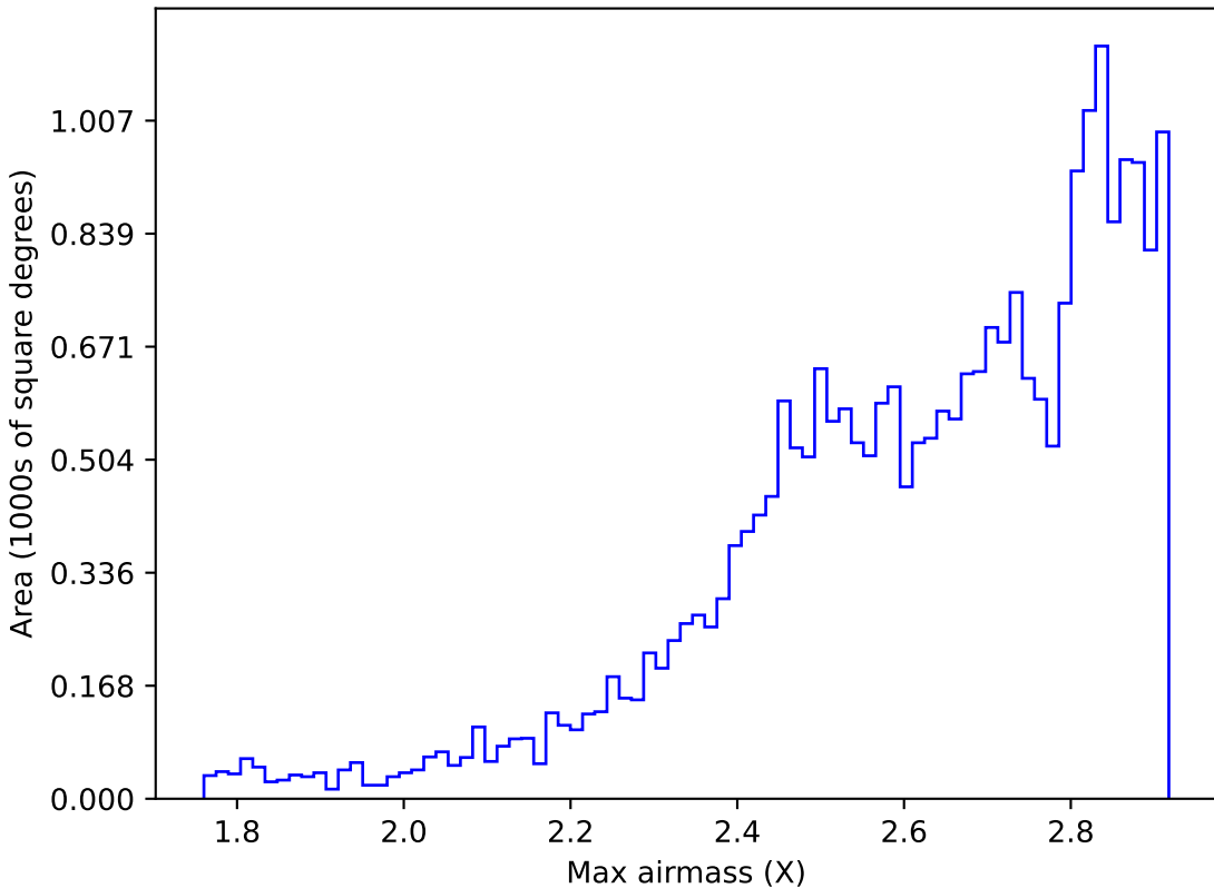
too_5_1v3.4_10yrs All sky all bands: Max airmass
