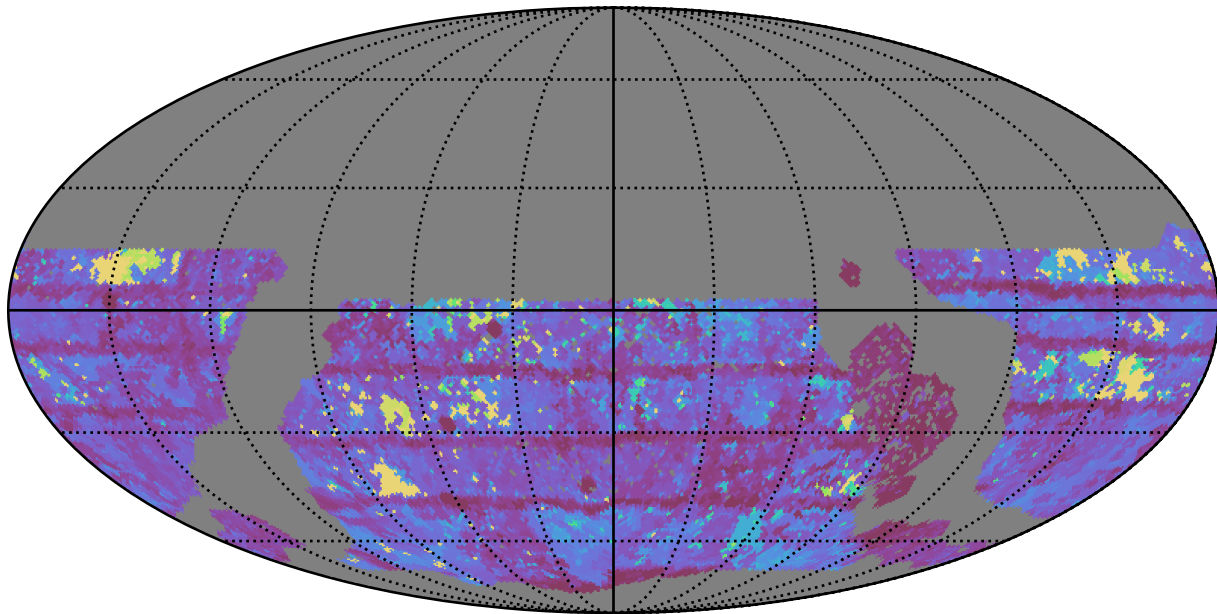
too_5_1v3.4_10yrs WFD z band: Max Inter-Night Gap
