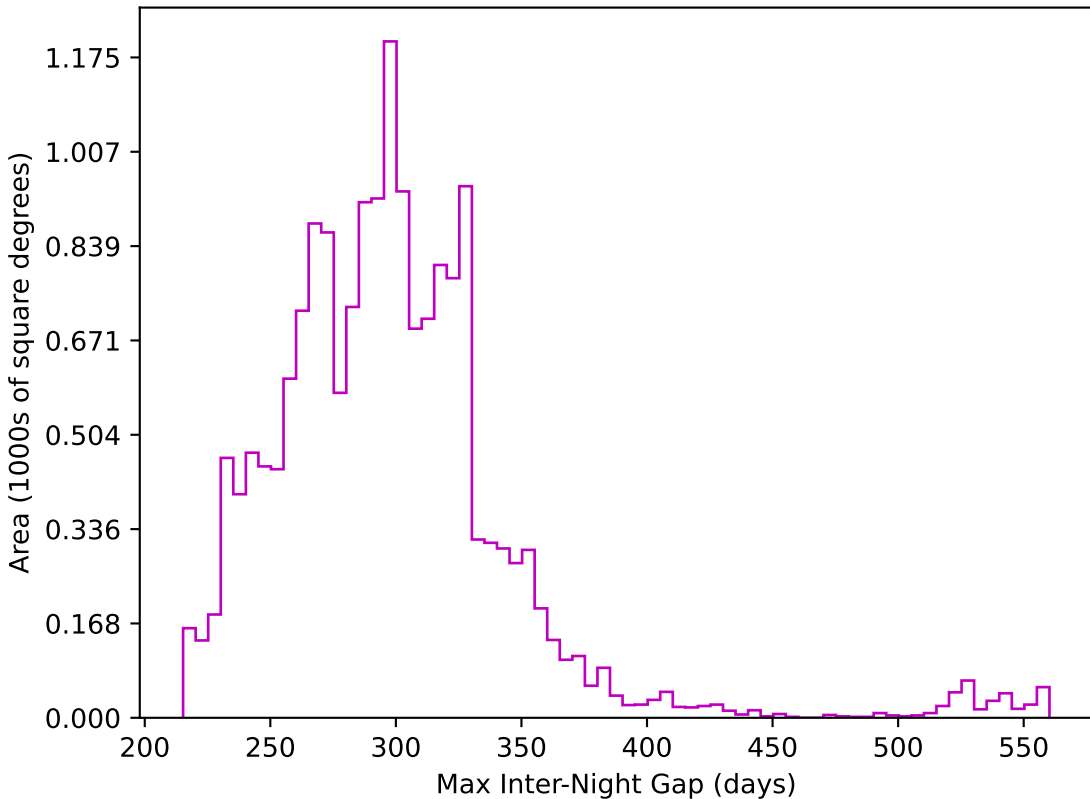
too_5_1v3.4_10yrs WFD z band: Max Inter-Night Gap
