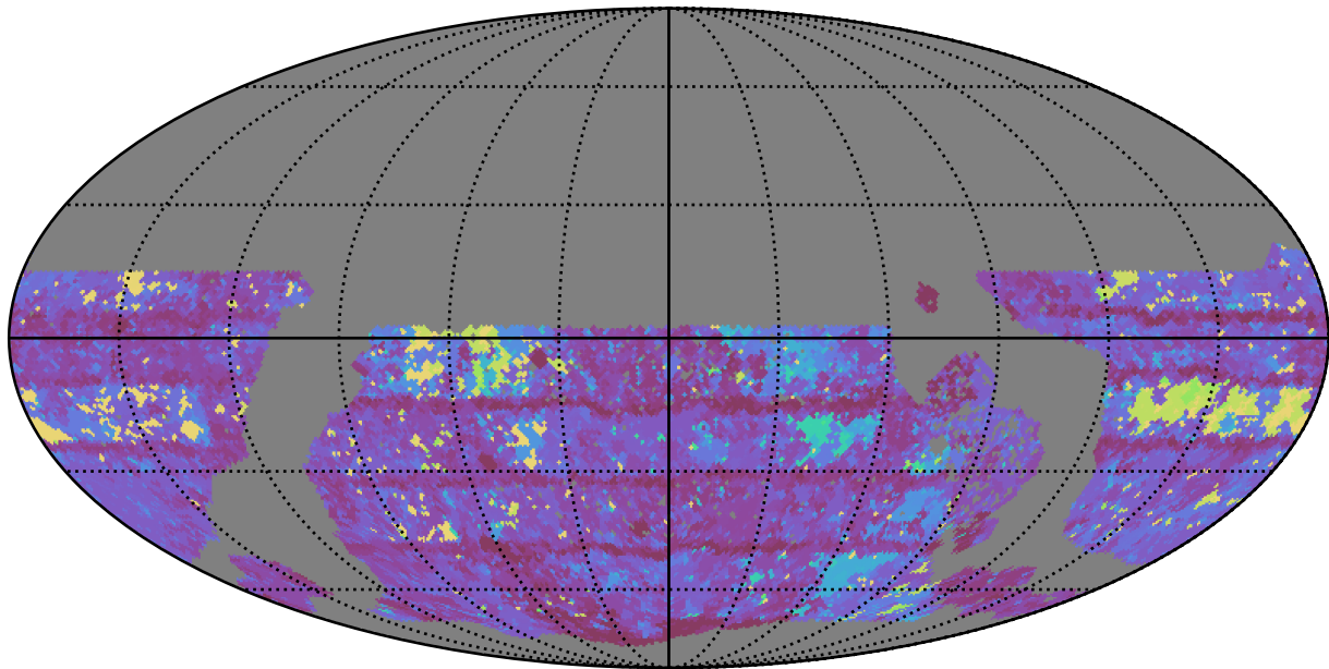
too_5_1v3.4_10yrs WFD y band: Max Inter-Night Gap
