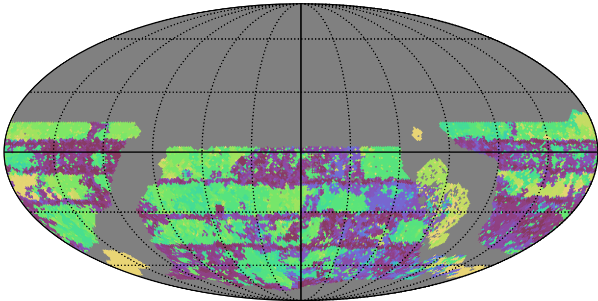
too_5_1v3.4_10yrs WFD u band: Max Inter-Night Gap
