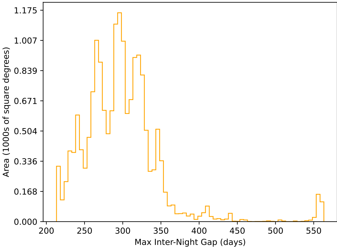
too_5_1v3.4_10yrs WFD r band: Max Inter-Night Gap
