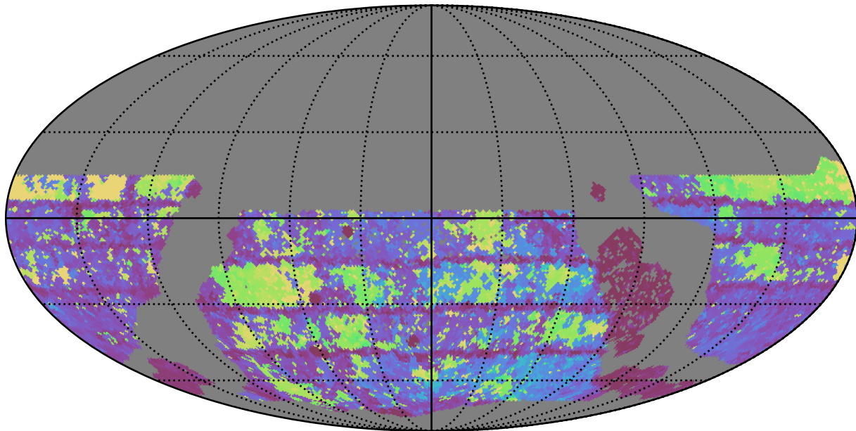
too_5_1v3.4_10yrs WFD g band: Max Inter-Night Gap
