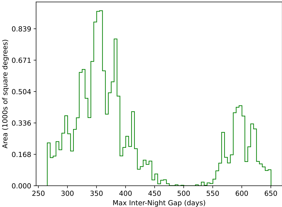
too_5_1v3.4_10yrs WFD g band: Max Inter-Night Gap
