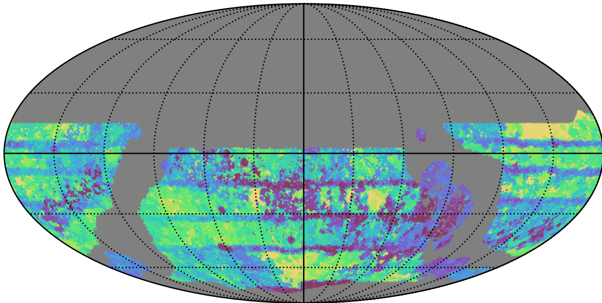
too_5_1v3.4_10yrs WFD all bands: Max Inter-Night Gap
