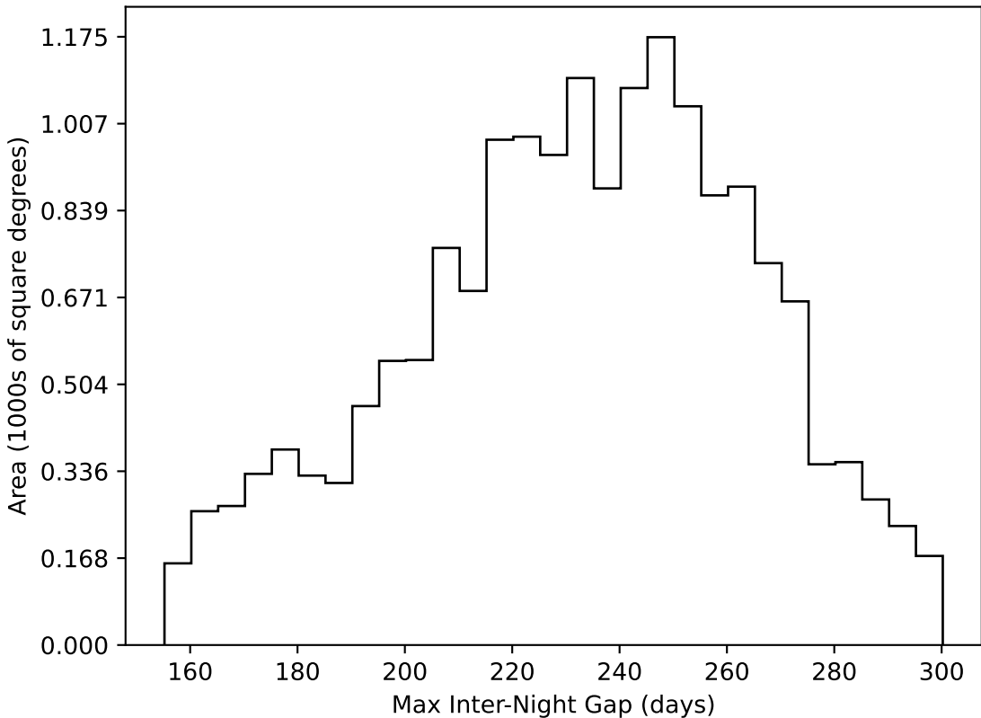
too_5_1v3.4_10yrs WFD all bands: Max Inter-Night Gap
