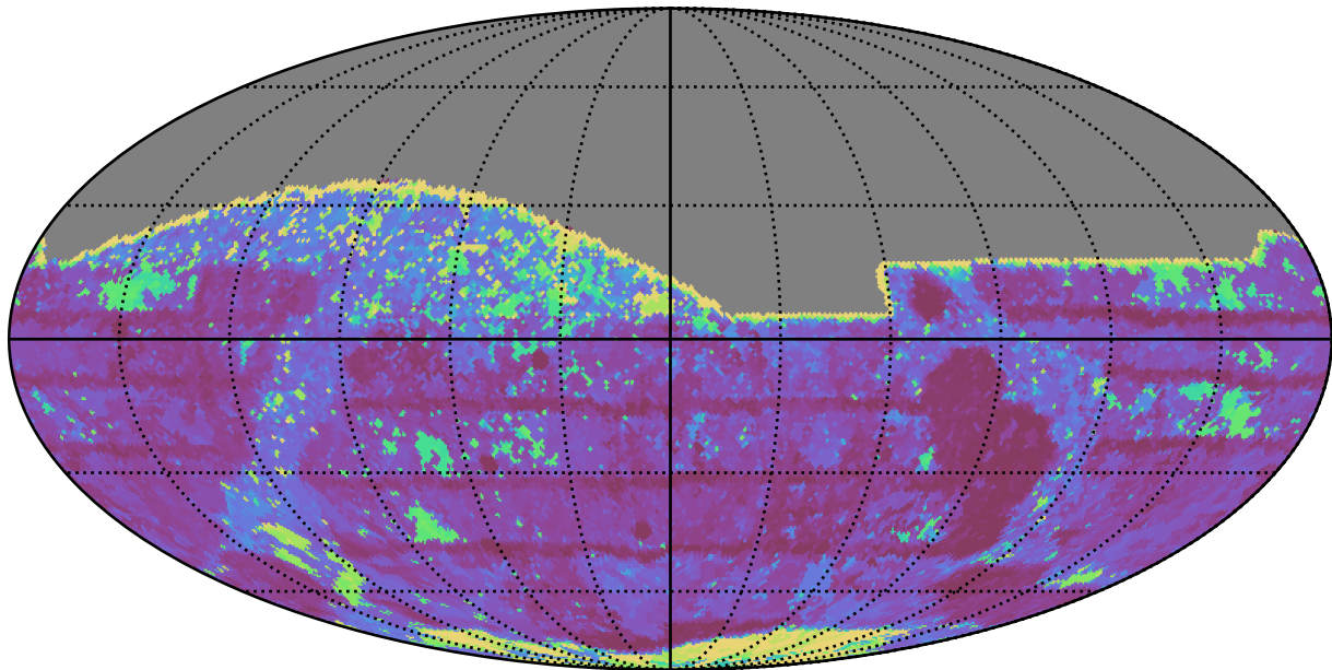
too_5_1v3.4_10yrs All sky z band: Max Inter-Night Gap
