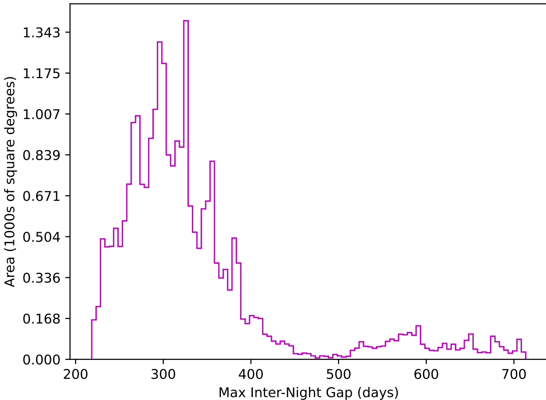
too_5_1v3.4_10yrs All sky z band: Max Inter-Night Gap
