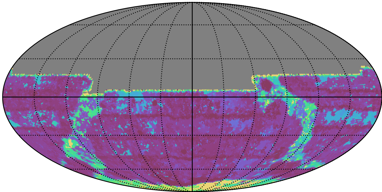
too_5_1v3.4_10yrs All sky y band: Max Inter-Night Gap
