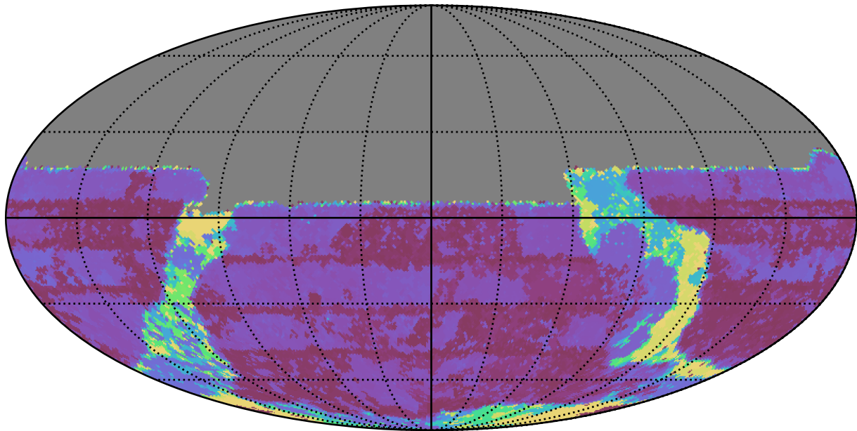
too_5_1v3.4_10yrs All sky u band: Max Inter-Night Gap
