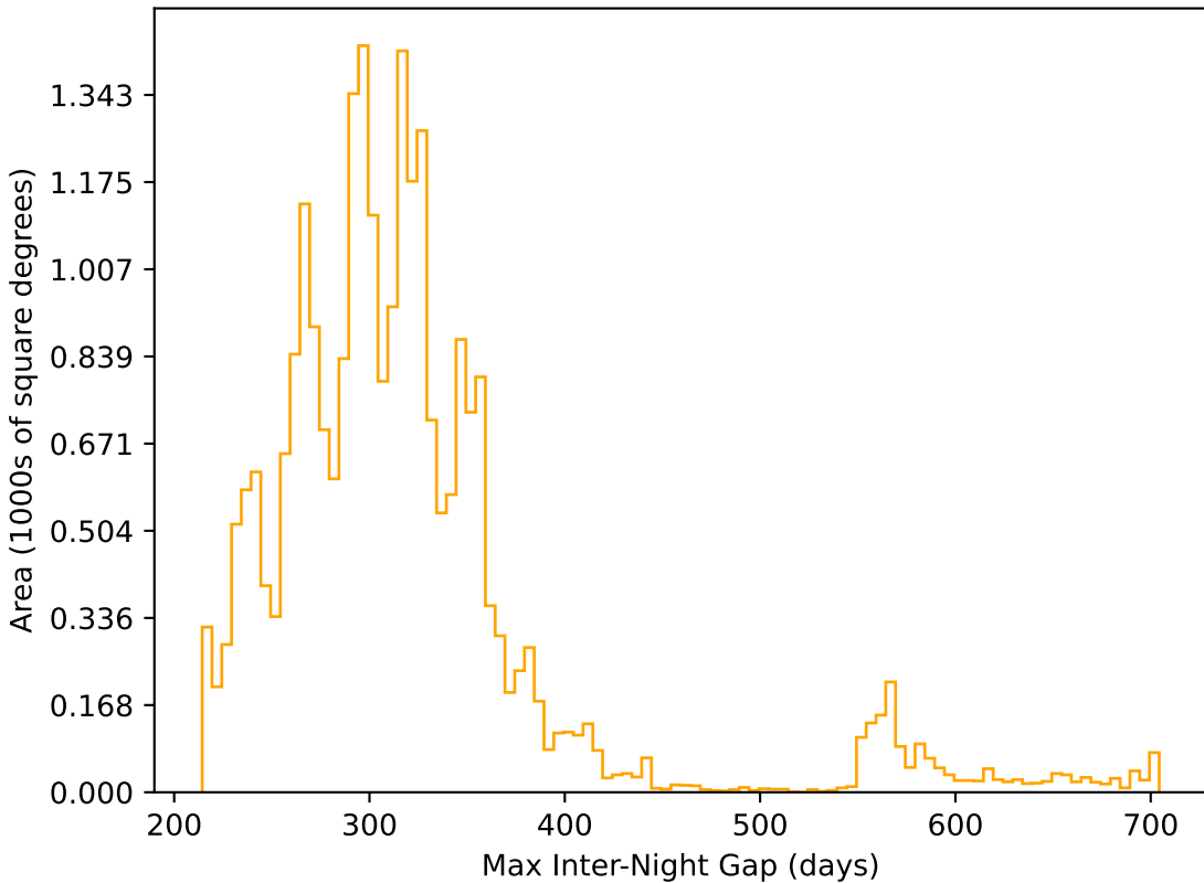
too_5_1v3.4_10yrs All sky r band: Max Inter-Night Gap
