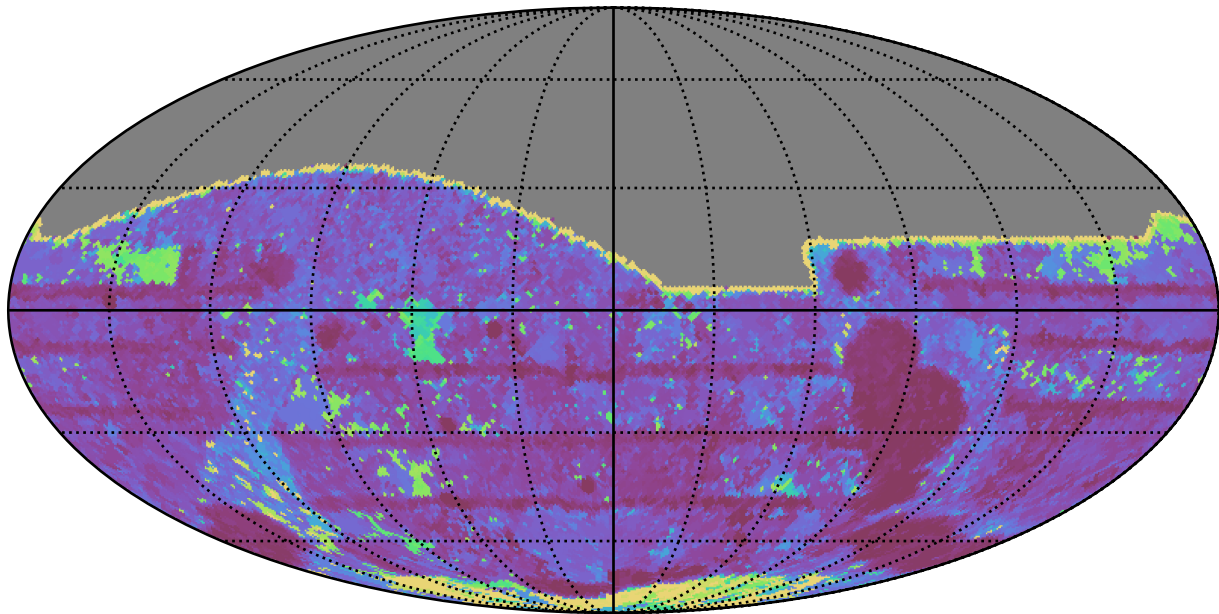
too_5_1v3.4_10yrs All sky i band: Max Inter-Night Gap
