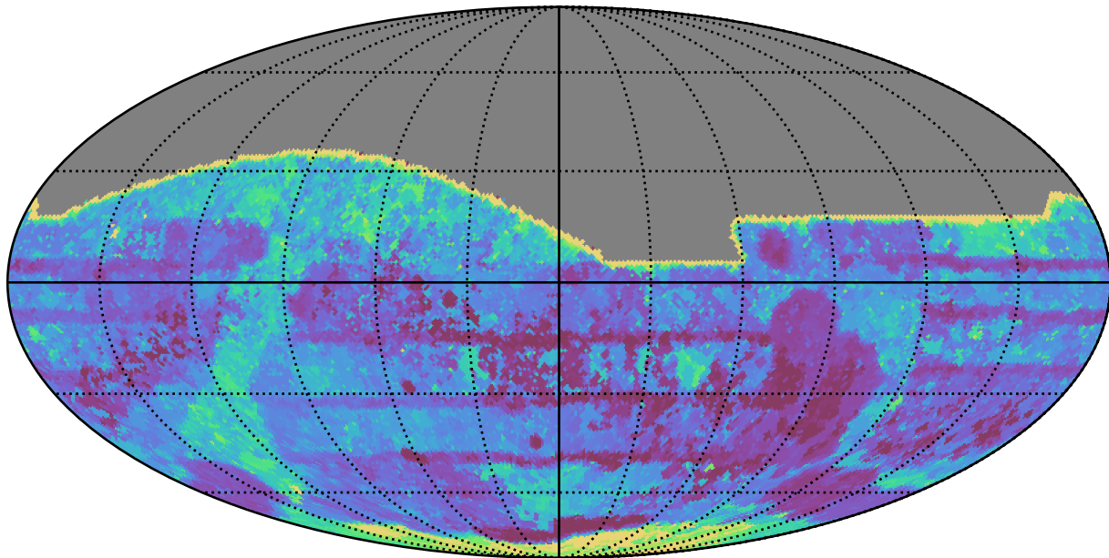
too_5_1v3.4_10yrs All sky all bands: Max Inter-Night Gap
