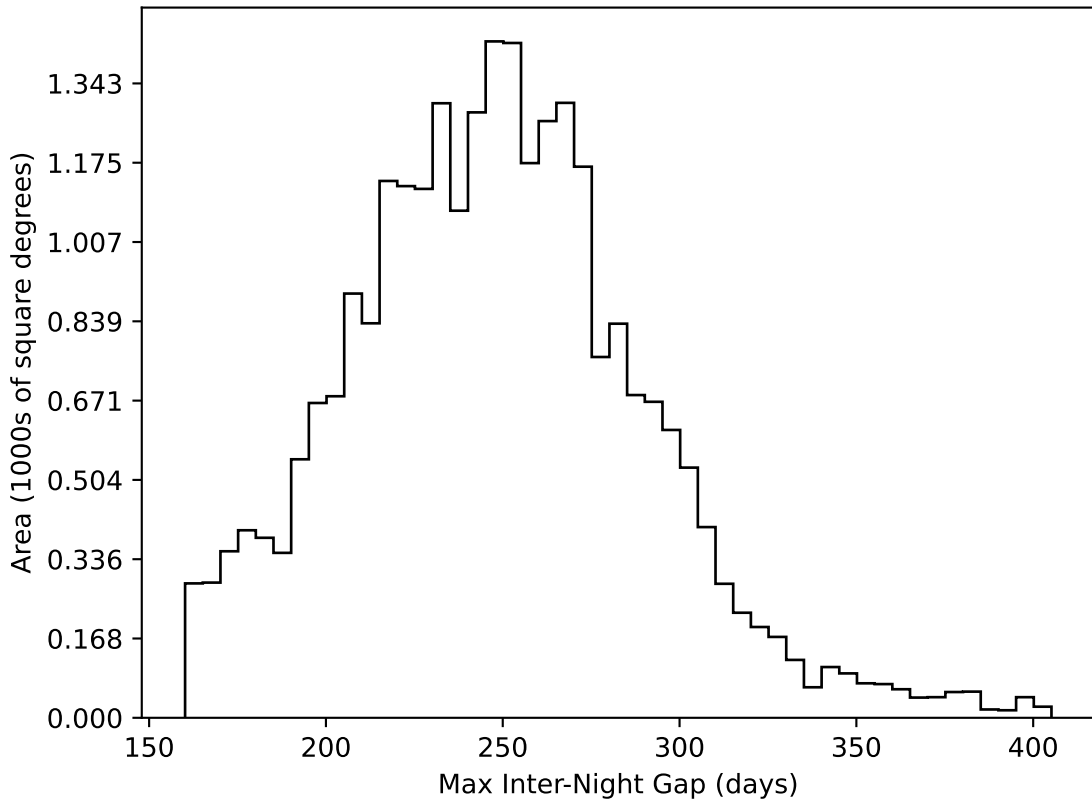
too_5_1v3.4_10yrs All sky all bands: Max Inter-Night Gap
