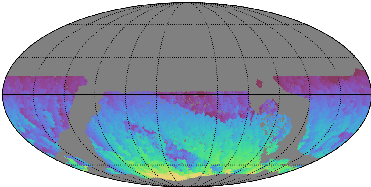
too_5_1v3.4_10yrs WFD z band: Max HA
