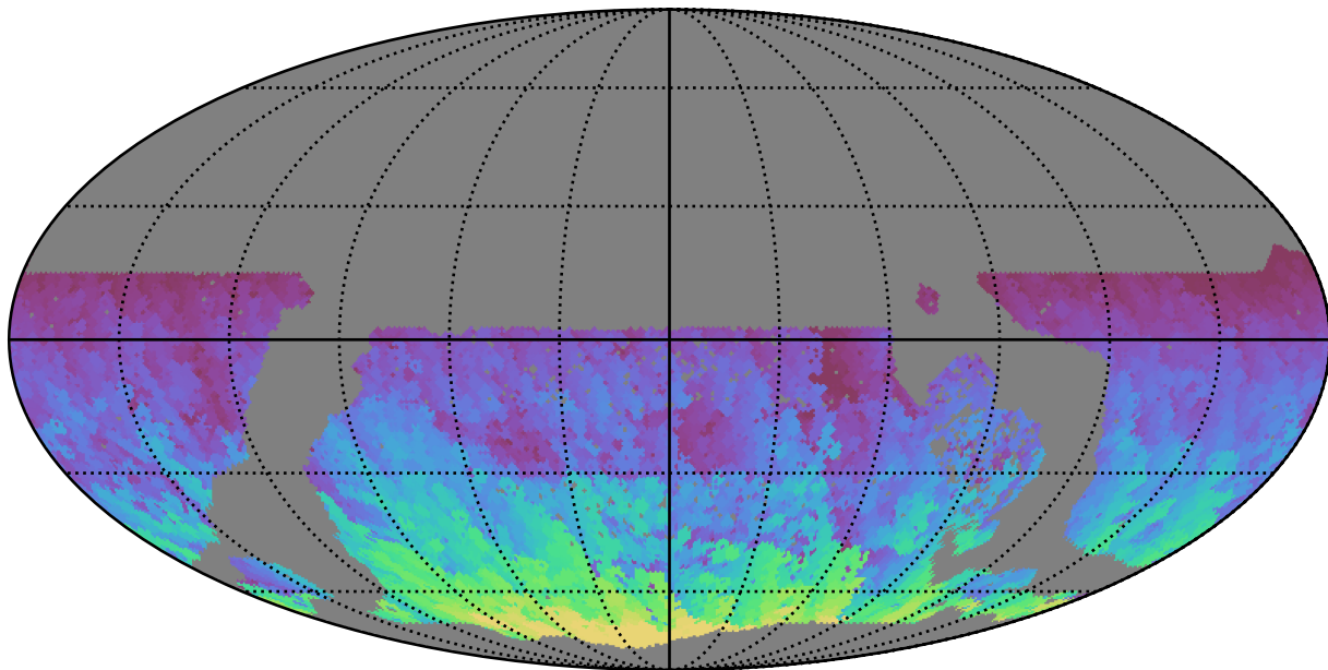
too_5_1v3.4_10yrs WFD y band: Max HA
