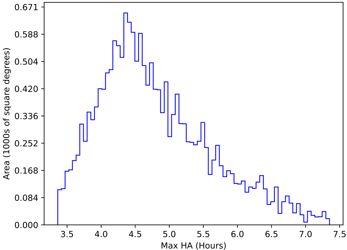
too_5_1v3.4_10yrs WFD y band: Max HA
