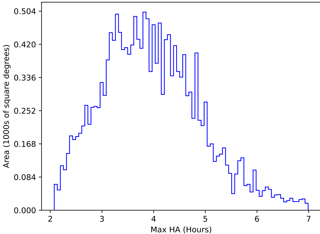
too_5_1v3.4_10yrs WFD u band: Max HA
