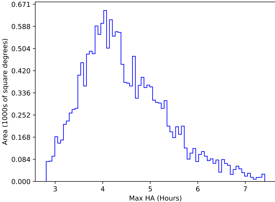
too_5_1v3.4_10yrs WFD r band: Max HA
