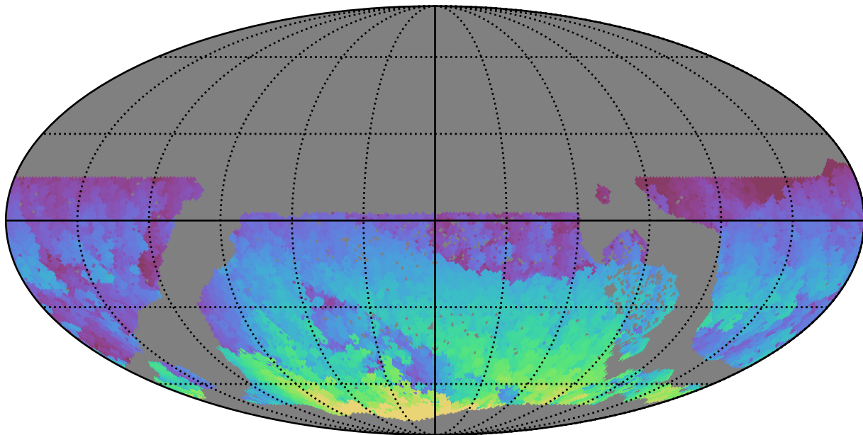
too_5_1v3.4_10yrs WFD i band: Max HA
