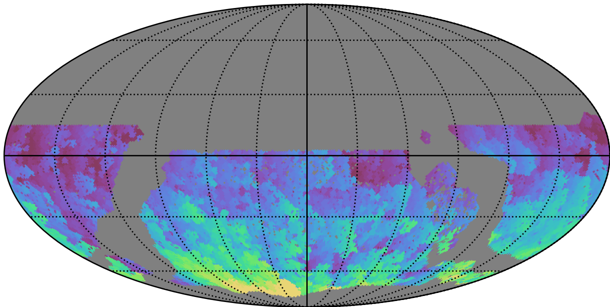
too_5_1v3.4_10yrs WFD g band: Max HA
