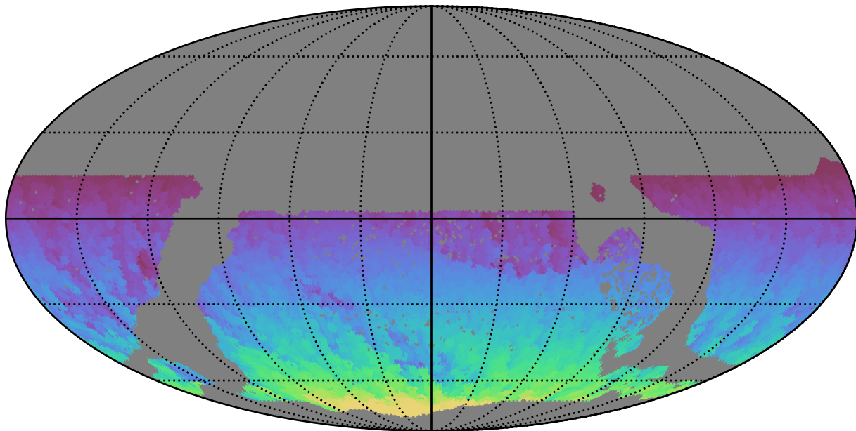
too_5_1v3.4_10yrs WFD all bands: Max HA
