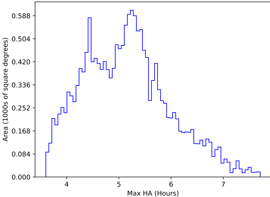
too_5_1v3.4_10yrs WFD all bands: Max HA
