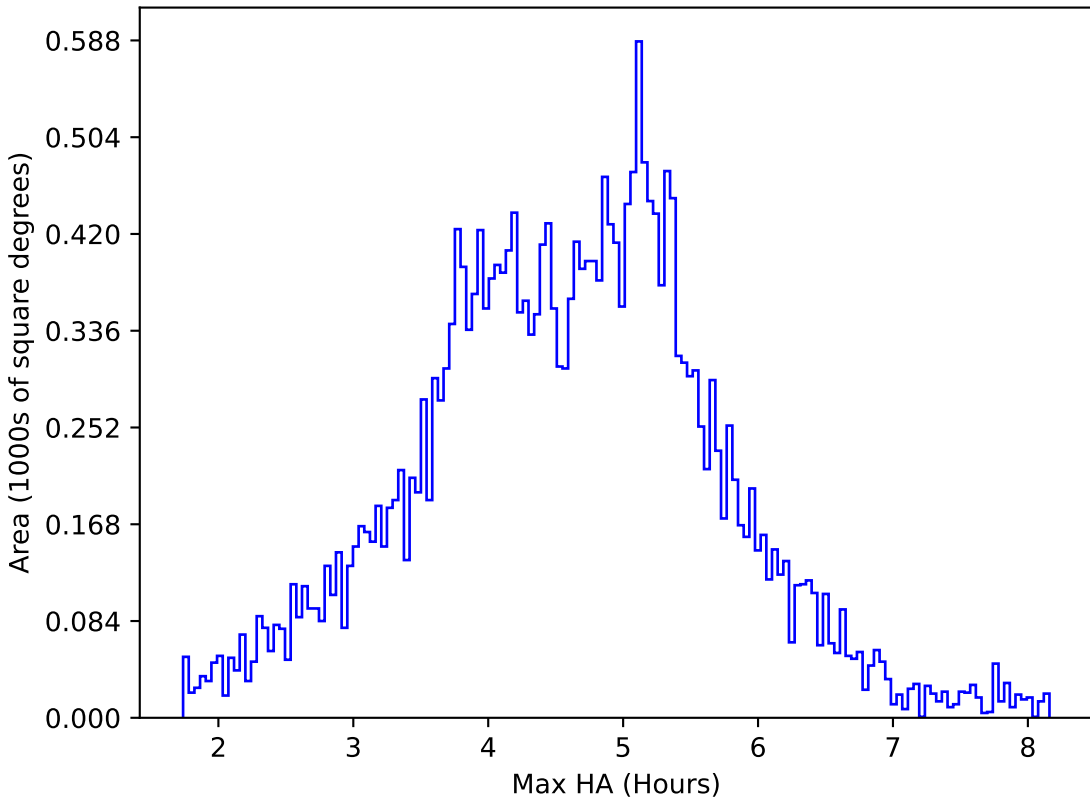
too_5_1v3.4_10yrs All sky z band: Max HA
