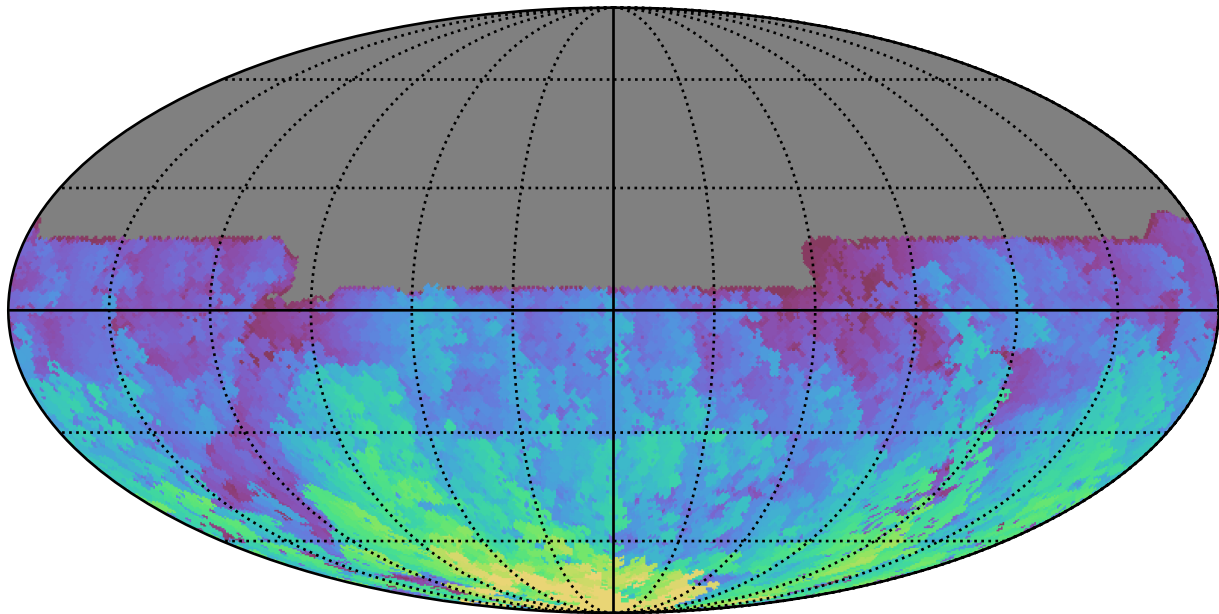
too_5_1v3.4_10yrs All sky u band: Max HA
